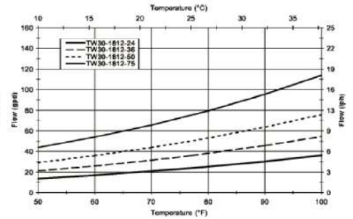
Figure 2: Impact of Temperature on Permeate Flow (constant temperature, recovery)
