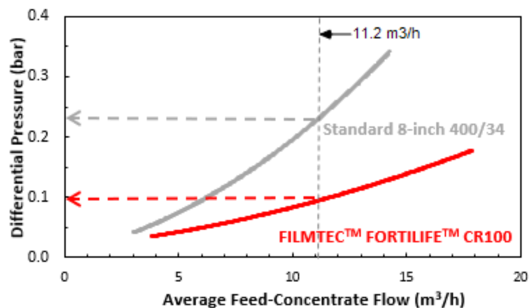
Figure 1: Element differential pressure as a function of flow rate for FILMTEC™ FORTILIFE™ CR100 elements vs. standard elements
